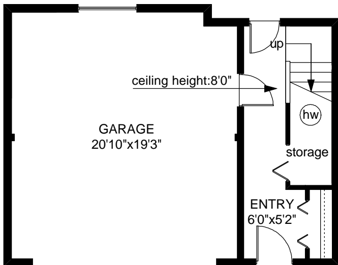
LOWER FLOOR 167 SQ.FT
