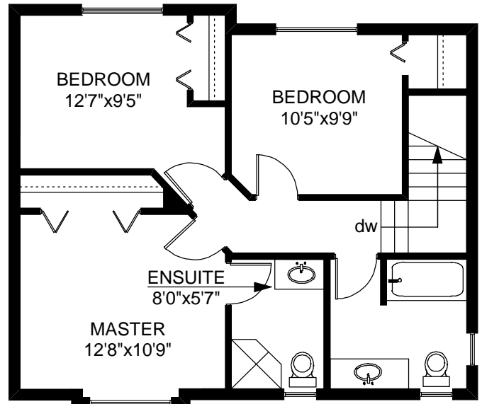
UPPER FLOOR 648 SQ.FT
