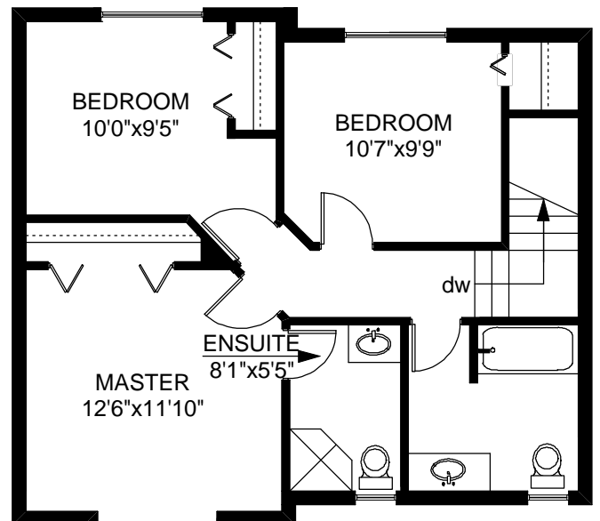
UPPER FLOOR 654 SQ.FT
